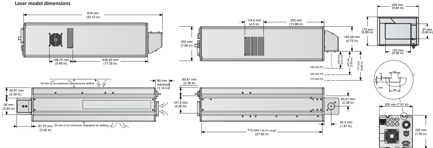
Laser model dimensions
